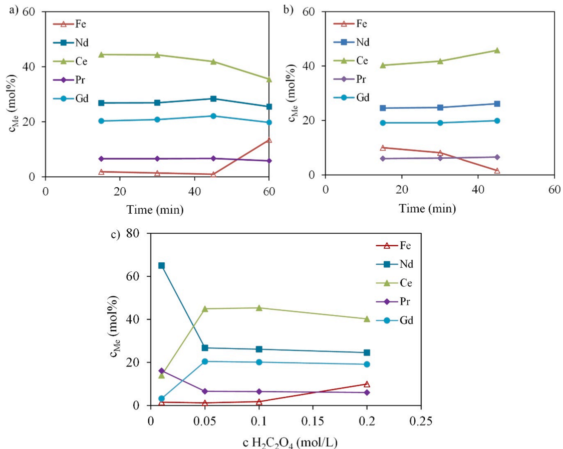
Fig. 4. Concentration of metal ions in the oxalate precipitate depending on leaching time in 0.5 mol/L \text{H}_2\text{SO}_4 containing (a) 0.1 mol/L \text{H}_2\text{C}_2\text{O}_4 and (b) 0.2 mol/L \text{H}_2\text{C}_2\text{O}_4 ; (c) concentration of oxalic acid (after 15 min of electrolysis).
