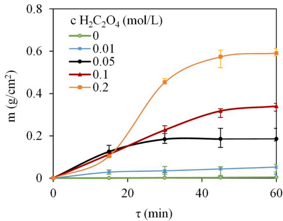
Fig. 3. Precipitation of REE oxalates during electro-leaching of NdCeFeB magnet in 0.5 mol/L \text{H}_2\text{SO}_4 solutions with different concentrations of oxalic acid, i_a = 50 \text{ A/dm}^2 .
