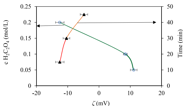
Fig. 5. Dependence of zeta potential of the oxalate precipitate on the concentration of oxalic acid at t = 15 min and on leaching time at c_{\text{H}_2\text{C}_2\text{O}_4} = 0.2 M.
