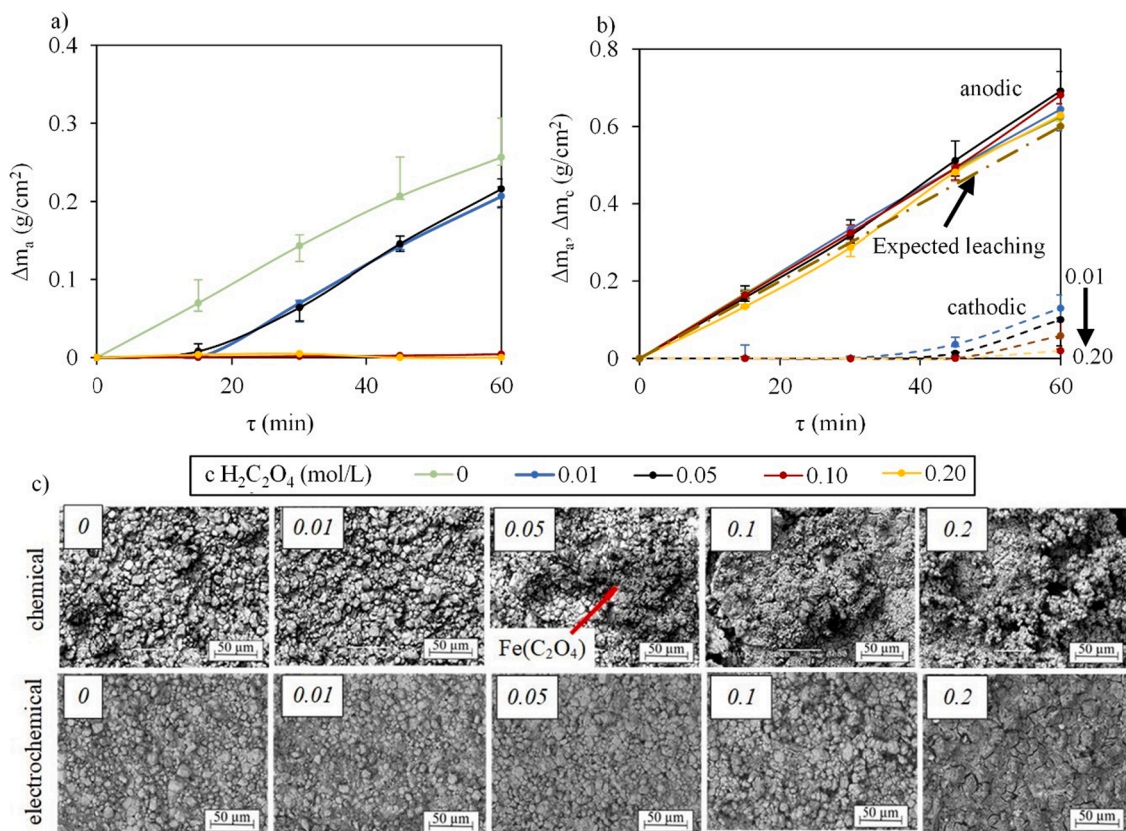
Fig. 6. Weight loss of NdCeFeB magnets during chemical leaching (a) and electro-leaching (b) in 0.5 mol/L \text{H}_2\text{SO}_4 with different concentrations of oxalic acid. Dashed lines correspond to weight increase on cathode due to iron reduction and the numbers indicate oxalate concentration. i_a = 50 \text{ A/dm}^2 . Surface scans (c) were taken after 60 min of leaching. Expected electrochemical leaching corresponds to theoretical leaching value calculated by the Faraday's law.
