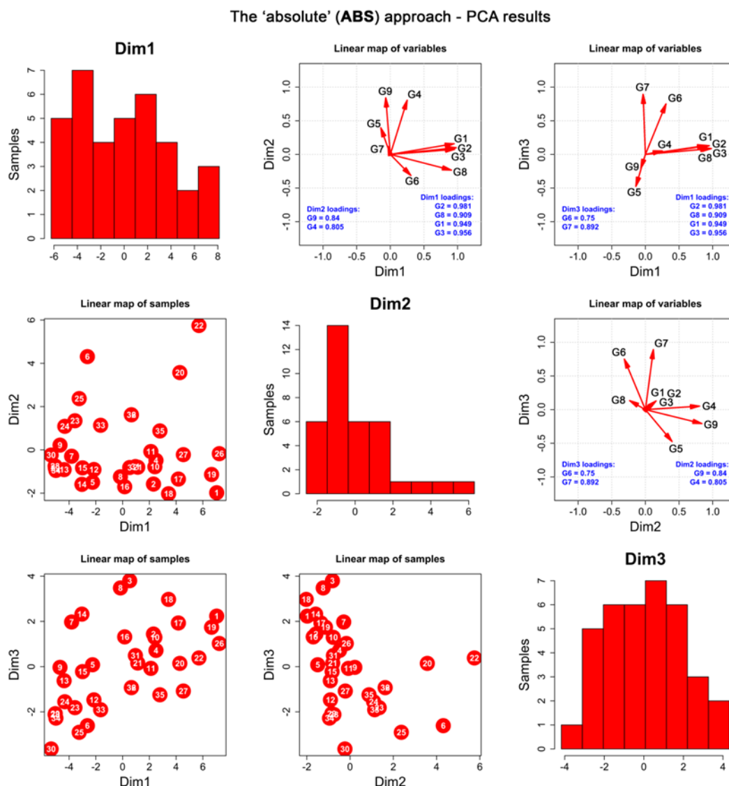
Figure 2. PCA performed for the ABS dataset. Diagonal: histograms of the first three resulting PCs subjected to VARIMAX rotation (henceforth known as dimensions, Dim). Lower triangle: linear maps of samples in the space of the first three dimensions. Upper triangle: linear maps of original variables (compounds) in the space of the first three dimensions. The numbers correspond to the numbering presented in the Section 3.1.
