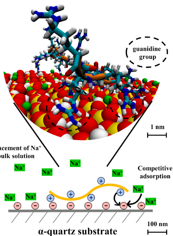
Fig. 7. Schematic illustration of competitive adsorption between the PP and \text{Na}^+ ions on \alpha -quartz surface and MD simulation snapshot of PARG at pH = 10.0. The atomistic detail level model highlights the ion exchange mechanism with no \text{Na}^+ ions in the close vicinity of guanidine groups that are interacting with the surface.
